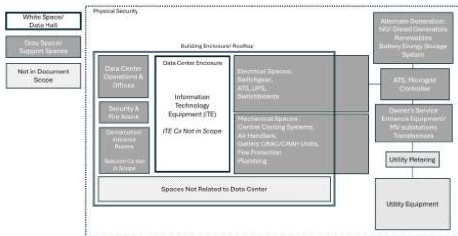
Figure 4-1 Demarcation of systems and building areas within the scope of this guideline.
