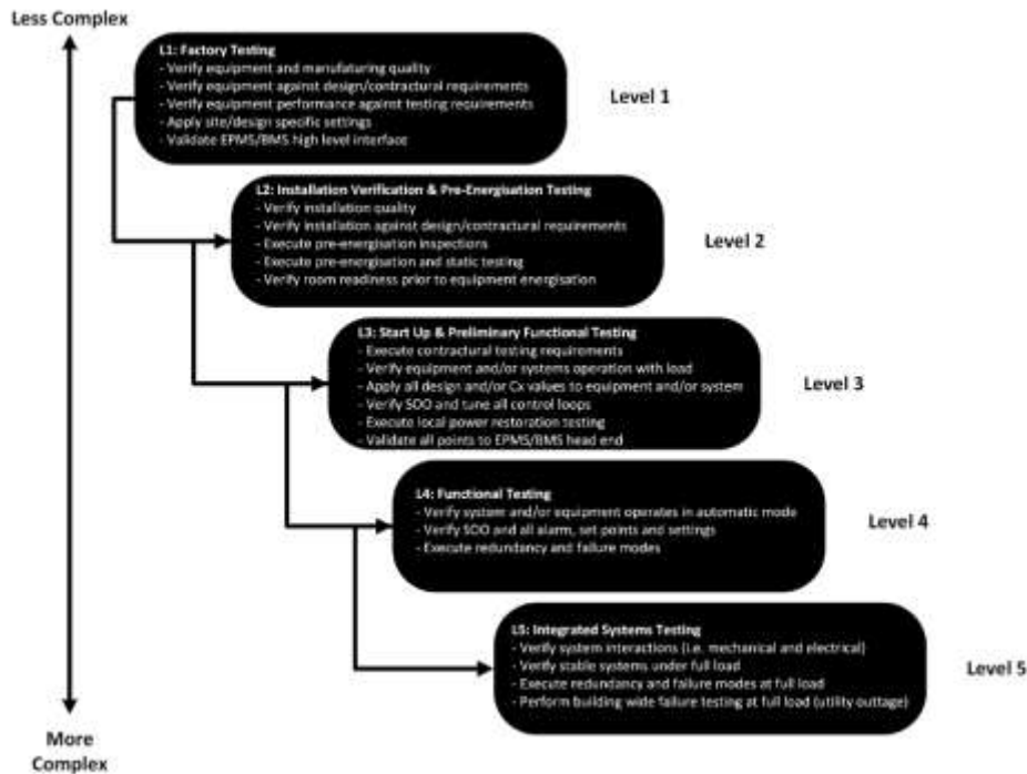
Figure 6-1 Levels of Commissioning.
